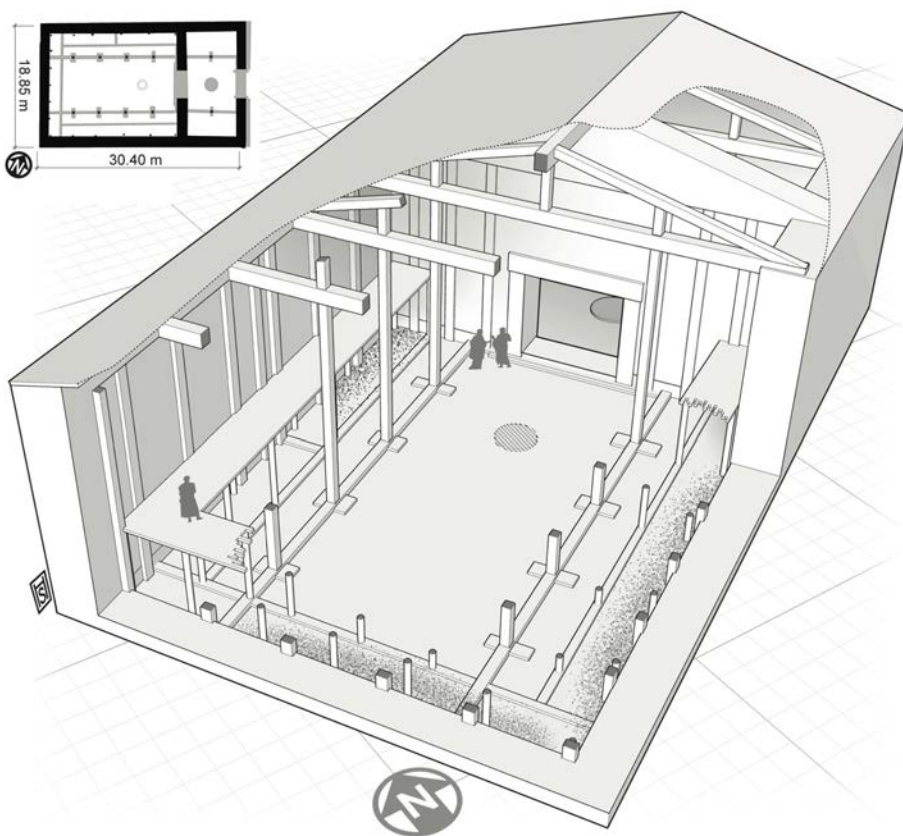
Figure 4: Reconstruction of the interior of Megaron 3 in the late 9th century BCE, with human scale. Drawing by Samuel Holzman.
